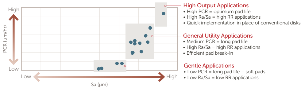
Pad Cut Rate (PCR) vs Surface Roughness (Sa) [IC1000]
