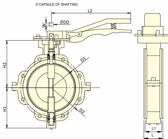
D CAPSULE OF SHAFTING
